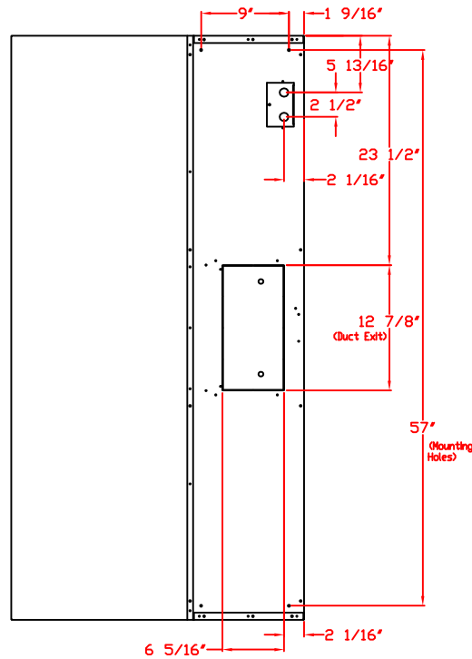
TOP VIEW (DUCT EXIT SHOWN IN TOP LOCATION)
